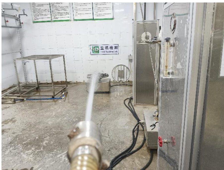
Photo 4: IPX5 test of model 2835-180L-230V-4000K
