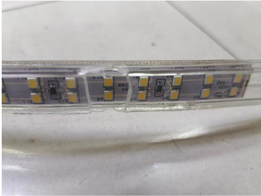
Photo 7: Test result of IP6X and IPX5 test
